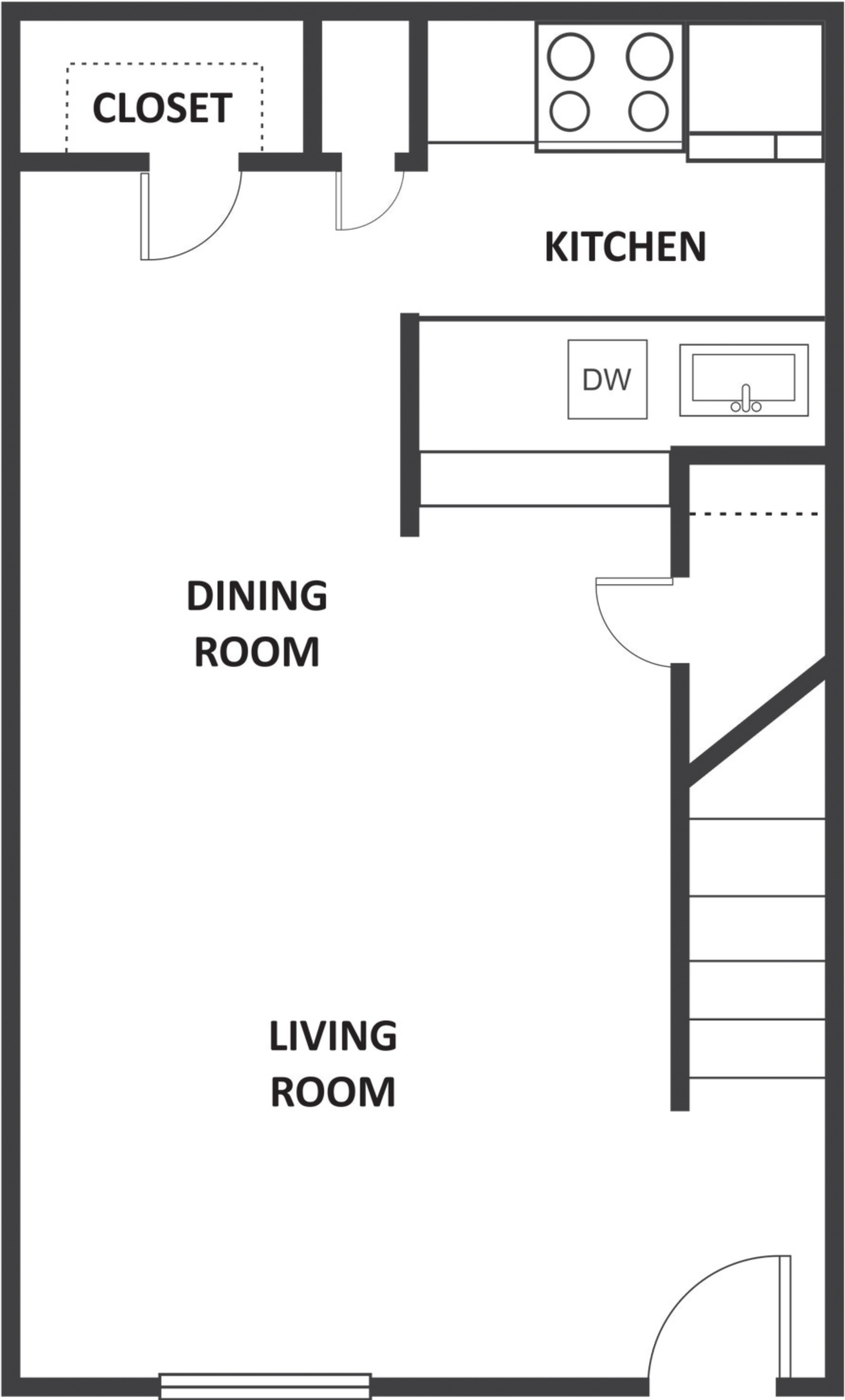
FLOOR1
